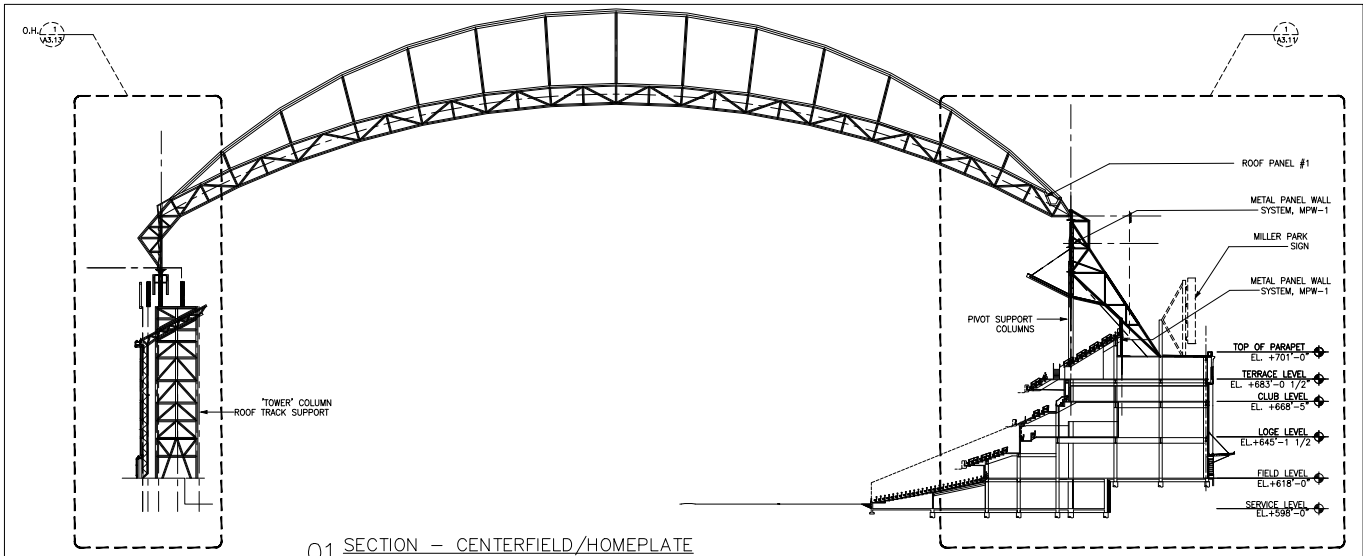
01 SECTION - CENTERFIELD/HOMEPLATE SCALE: 1/32" = 1'-0"
