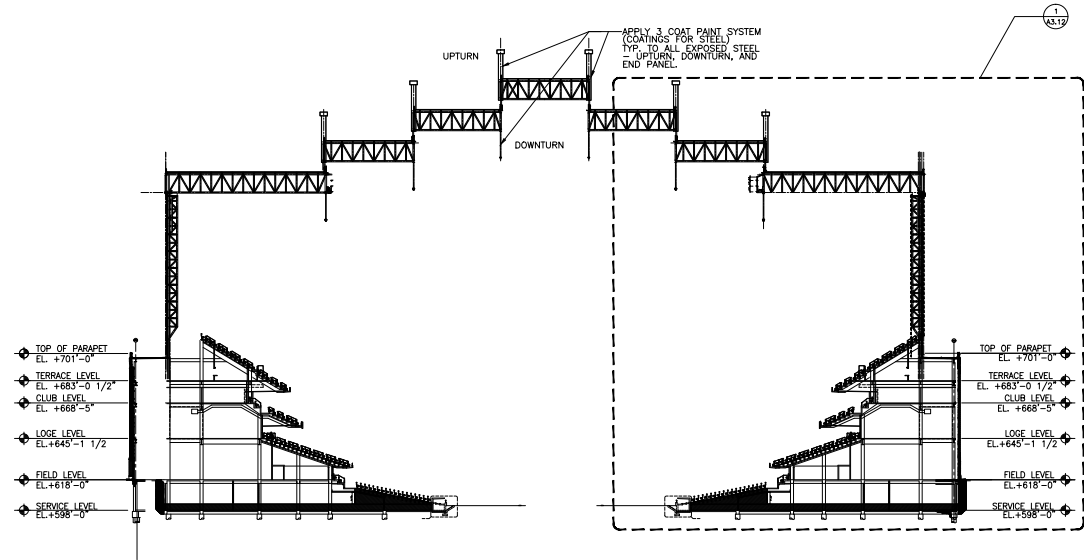
02 SECTION - FIRST BASE/THIRD BASE SCALE: 1/32" = 1'-0"
