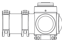
QSM Mounting with PR3E or PR7E option
