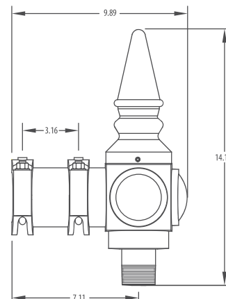
NPT15R Mounting
