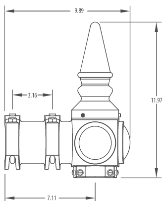
QSM Mounting
