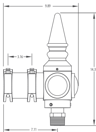
NPT15S Mounting
